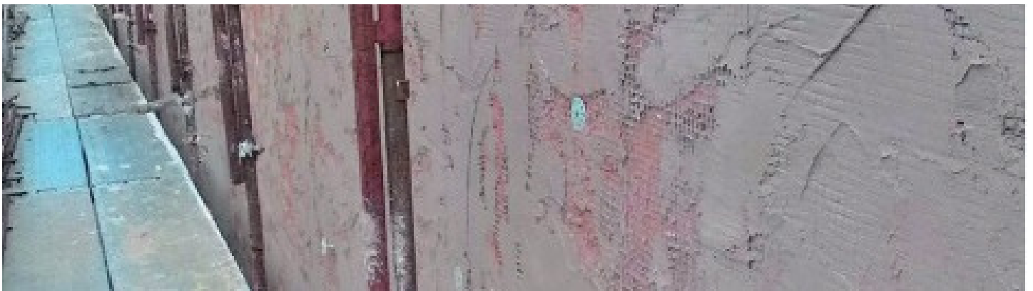
Application of an overcoat mesh with a first coat of Stabilitura Naturale Traspirante Plus
