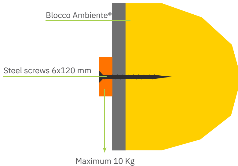
Support details for light loads
