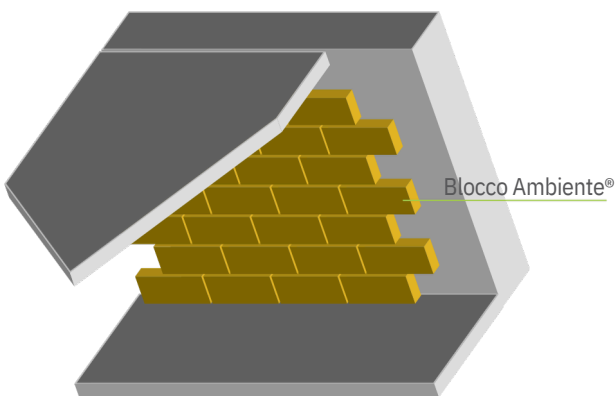
Fig.3 Insulating counterwall
