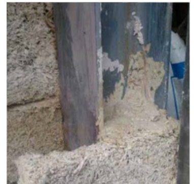
Blocco Ambiente ® shaped block used to solve the thermal bridge from the structural frame
