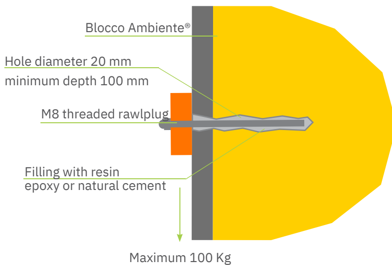
Support detail for heavy loads
